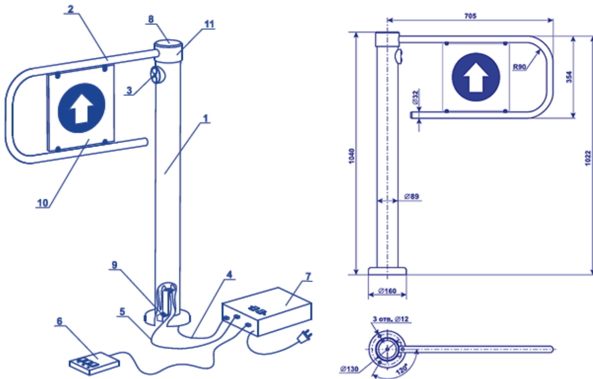
1 - gate post; 2 - swing panel; 3 - indication module; 4 - power cable; 5 - control cable; 6 - remote control panel with cable; 7 - switching and power unit (SPU); 8 - cover; 9 - M8 bolt; 10 - double - sided info sign with fasteners; 11 - rotation unit.
