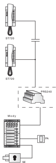
Intercoms connected to 1 external door station, traditional intercom system
