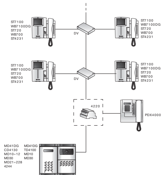
Digital videointercom system with 1 entrance and videointercoms with integrated decode module
