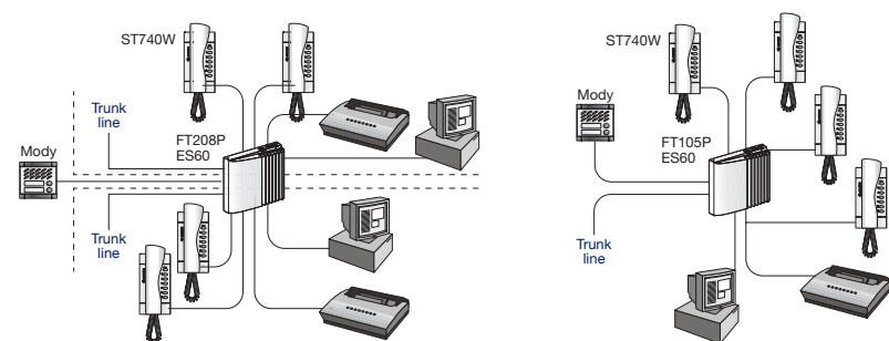
Examples of systems with intercom-telephone-set and PABX's
