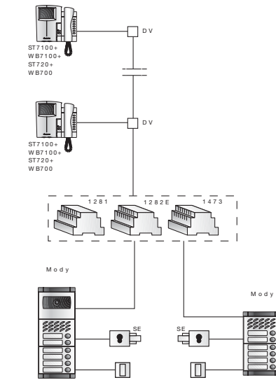
Multi-way videointercom system with 2 automatically switched entrances, one of which only audio, traditional system
